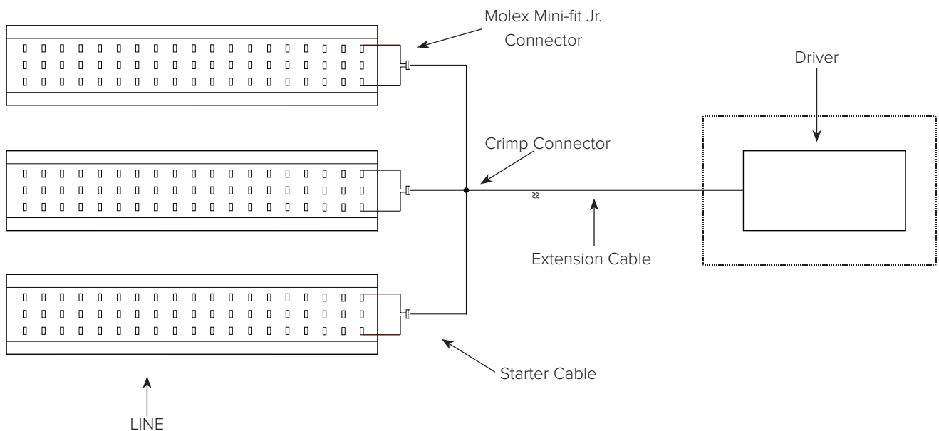
Multiple LINE Sheets wired to LED Driver
